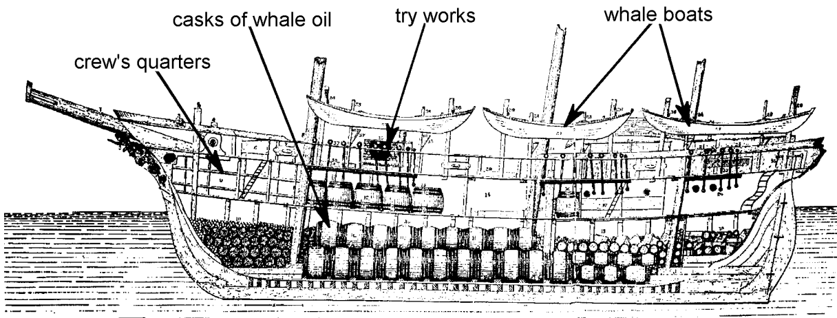
A cut away view of the Alice Knowles , a New Bedford sailing bark
